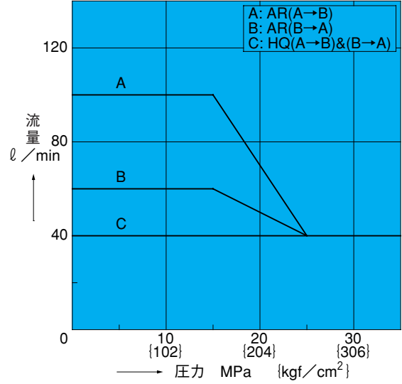
SNH-G06-AR/HQ
