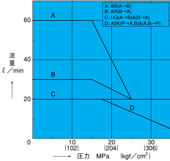
SNH-G04-AR/HQ
